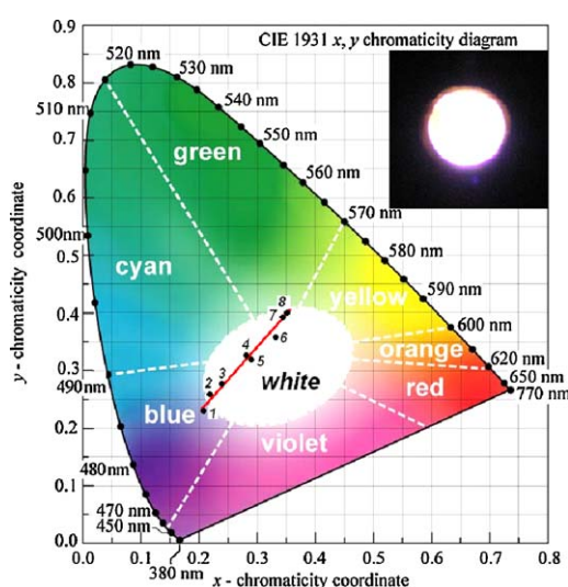
Figure 14 (x, y) chromaticity diagram of white emitting CdS nanoluminophores tuned with their amount hybridized on the LED [35].
