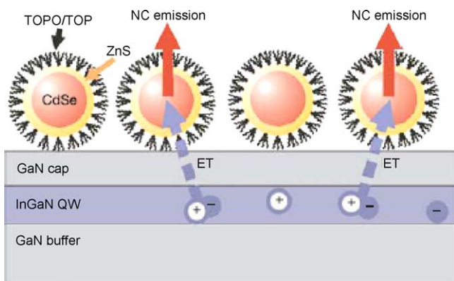
Figure 16 Schematic of the hybrid quantum-well/nanocrystal structure. The structure consists of an InGaN/GaN quantum-well heterostructure with a monolayer of TOPO/TOP-capped CdSe/ZnS core/shell nanocrystals on top of it. Electron–hole pairs generated in the quantum well can experience nonradiative energy transfer into the QDs by Förster-type, dipole–dipole interactions. The emission properties of the QDs excited by FRET are determined by the QD size. Reprinted by permission from MacMillan Publishers Ltd: Nature [44]. Copyright 2004.
