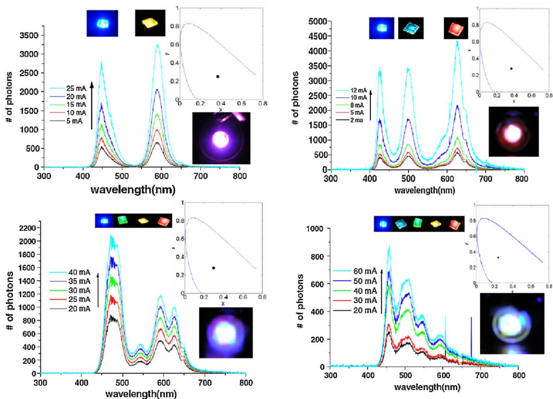
Figure 9 Luminescence spectra of (a) yellow-emitting QDs integrated on a blue LED at 440 nm, (b) cyan- and red-emitting QDs on the blue LED at 440 nm, (c) green-, yellow- and red-emitting QDs on the blue LED at 452 nm and (d) green-, cyan-, yellow- and red-emitting QDs on the blue LED at 452 nm at increasing current levels, and (x, y) coordinates of the hybrid white LED and pictures of the resulting hybrid white LED and used QDs [28].
