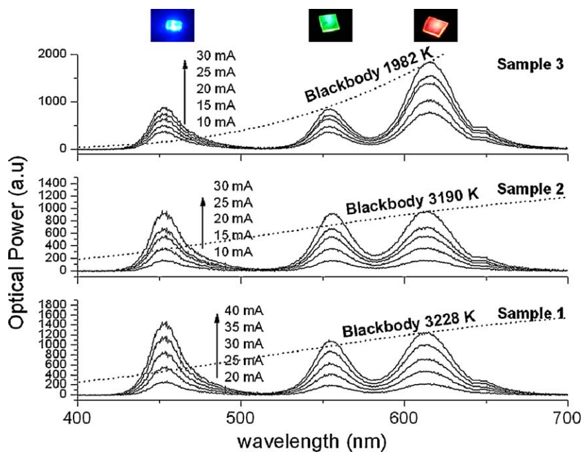
Figure 10 Luminescence spectra of Samples 1–3 at different current injection levels. Reprinted with permission from Reference [25]. Copyright 2008 American Institute of Physics.
