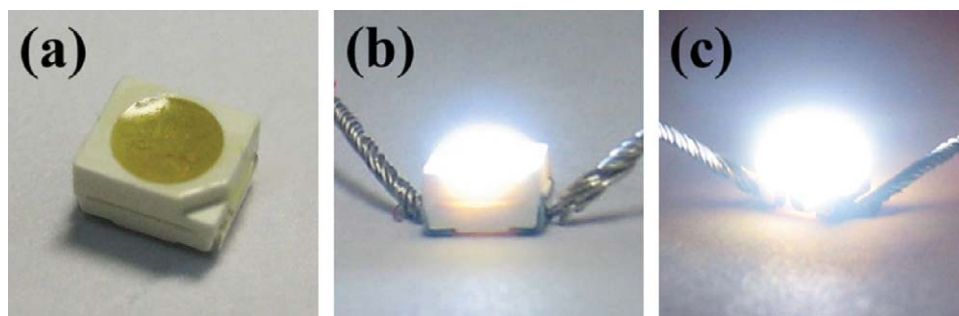
Figure 15 Photographs of (a) an as-prepared CdSe QD- and \text{Sr}_3\text{SiO}_5:\text{Ce}^{3+} , \text{Li}^+ phosphor-based white LED, (b and c) the same white light-emitting LED operated at 5 mA and 20 mA, respectively. Reprinted with permission from Reference [39]. Copyright 2008 WILEY-VCH Verlag GmbH & Co. KgaA, Weinham.
