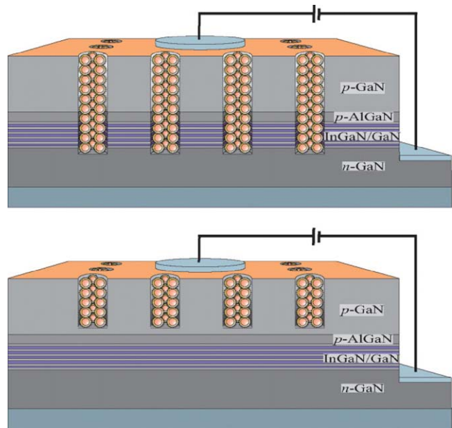
Figure 18 Schematic diagrams of the hybrid QD-LED etched to different levels: through the MQW (top) and only down to the p-AlGaIn layer (bottom). Reprinted with permission from Reference [49]. Copyright 2010 WILEY-VCH Verlag GmbH & Co. KgaA, Weinham.
