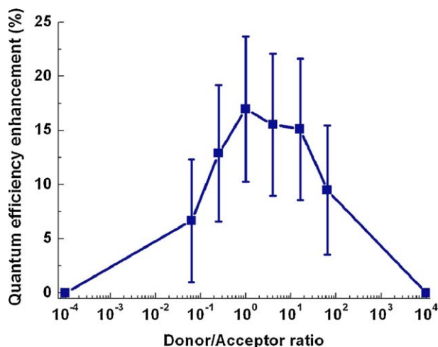
Figure 21 QD donor–acceptor ratio dependent quantum efficiency enhancement of the donor–acceptor hybrid solid films consisting of cyan- and green-emitting CdSe/ZnS core/shell QDs. Reprinted with permission from Reference [51]. Copyright 2009 American Institute of Physics.
