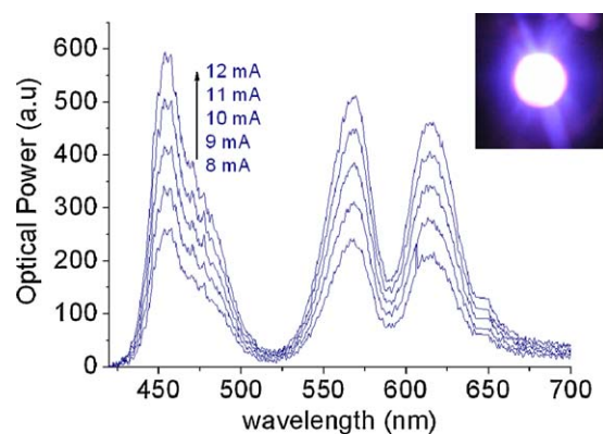
Figure 13 Luminescence spectra of onion-like CdSe/ZnS/CdSe core/shell/shell heteronanocrystals hybridized on a blue light emitting diode driven at different levels of current injection at room temperature, along with a picture of the resulting hybrid QD-white LED while generating white light. Reprinted with permission from Reference [33]. Copyright 2008 American Institute of Physics.
