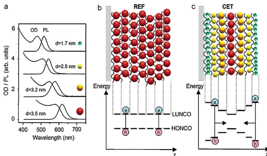
Figure 20 (a) Absorbance (optical density, OD) and photoluminescence (PL) spectra of the CdTe QDs of four different sizes used to prepare the layer-by-layer assembled samples. The sizes are chosen such that the emission spectrally matches the excitonic absorption of subsequently larger QDs. All spectra are taken in aqueous solution and vertically shifted for clarity. (b) Schematic sketch of the REF sample, which consists of seven layers of red-emitting, 3.5-nm large CdTe QDs. For the REF sample the energetic positions of the highest occupied nanocrystal orbital (HONCO) and the lowest unoccupied nanocrystal orbital (LUNCO) are sketched. Each excitation remains in the layer where it is created because of the absence of a gap gradient. (c) Sample CET consists of subsequent layers comprising green, yellow, orange, red, orange, yellow, and green-emitting QDs. For the CET sample the HONCO and LUNCO are also sketched, visualizing the cascaded band gaps used to facilitate cascaded energy transfer [50]. Reprinted with permission from Reference [50]. Copyright 2004 American Chemical Society.
