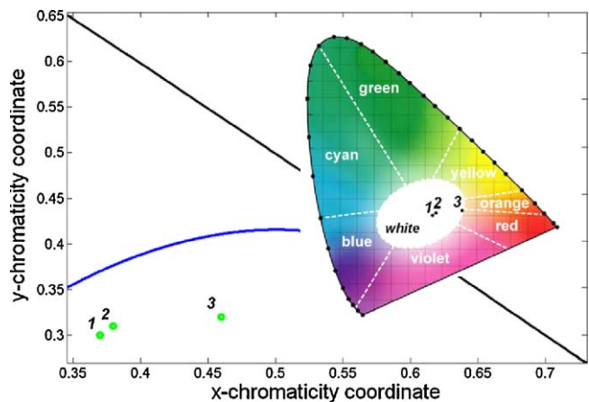
Figure 11 Zoomed (x, y) tristimulus coordinates of Samples 1–3. Blue curve denotes the Planckian locus (chromaticity points of the blackbody radiator) whereas the black line is the border of the (x, y) chromaticity diagram. The inset shows the (x, y) tristimulus coordinates on the CIE chromaticity diagram. Reprinted with permission from Reference [25]. Copyright 2008 American Institute of Physics.
