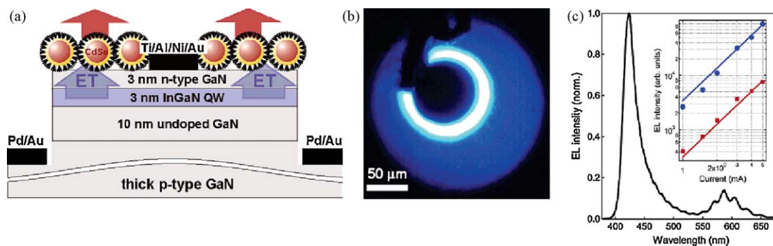
Figure 17 (a) Schematic cross section of the nonradiative energy transfer (ET)-LED structure, (b) LED under electrical excitation and (c) electroluminescence spectrum (2 mA driving current) displaying both QW (420 nm) and QD (590 nm) emission bands. Inset: QW (blue solid circles) and QD (red squares) emission intensities vs. driving current, indicating that the color-conversion efficiency (approximately the ratio of the two intensities) is independent of current [48]. Reprinted with permission from Reference [48]. Copyright 2006 American Chemical Society.
