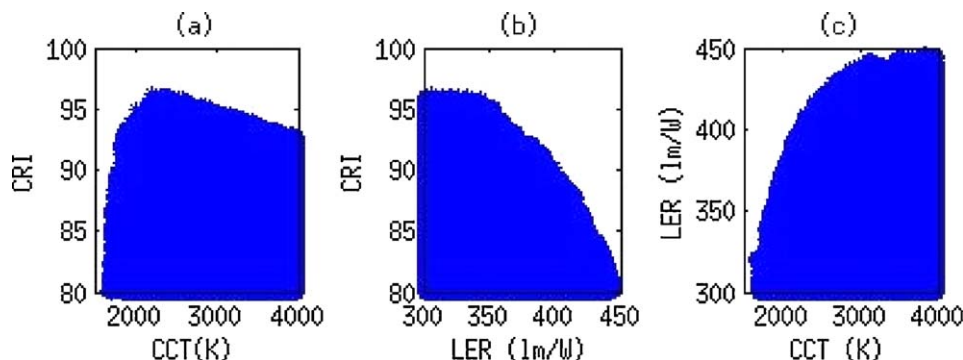
Figure 6 Relations between (a) CRI and CCT, (b) CRI and LER, and (c) LER and CCT [26].
