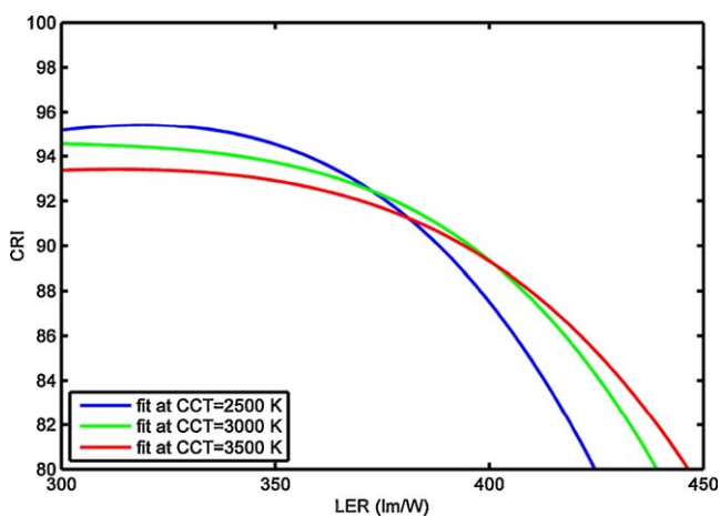
Figure 8 Feasibility of CRI vs. LER at different CCTs using quantum dot nanophosphors.
