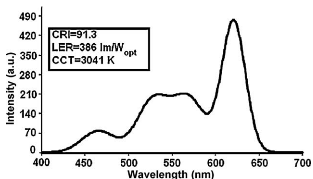
Figure 7 Exemplary spectrum generated using quantum dot nanophosphors (with the stated average values of the numerical analyses), together with the resulting photometric performance [26].
