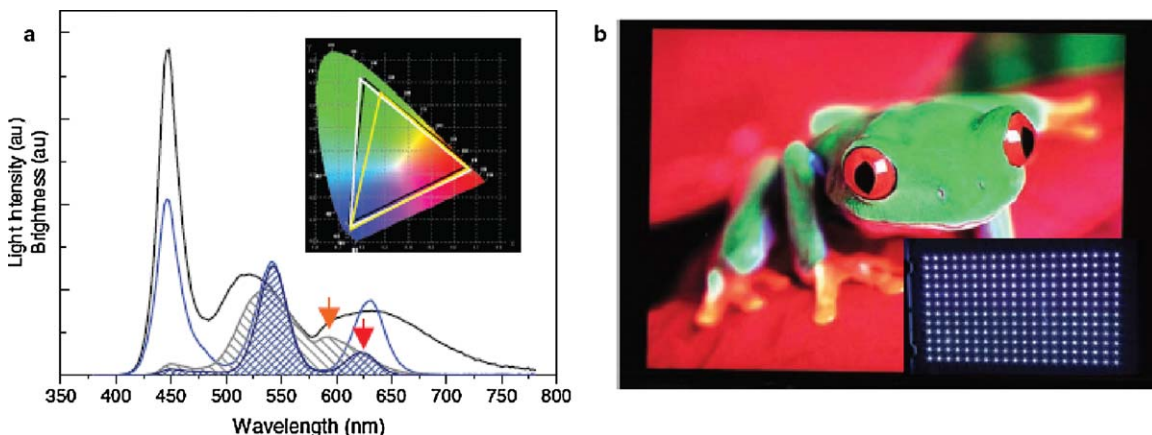
Figure 12 (a) Light intensity spectra (solid line) and brightness (hatched area) of the QD-LED (blue) and the phosphor-LED (grey). Inset: Color triangles of the QD-LED (white) and the phosphor-LED (yellow) compared to NTSC1931 (black). (b) A display image of a 46 inch LCD TV panel and a quarter of the white QD-LED backlights (inset). Reprinted with permission from Reference [31]. Copyright 2010 WILEY-VCH Verlag GmbH & Co. KgaA, Weinham.
