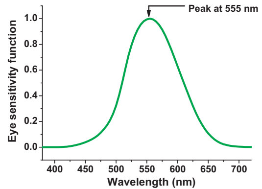
Figure 5 Eye sensitivity function spectrum (for light-adapted vision) [9].
