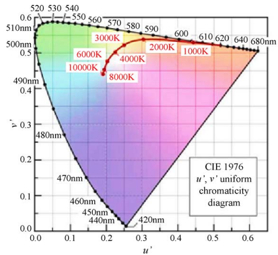
Figure 4 Chromaticity diagram ( u' , v' ) along with the Planckian locus [5].
