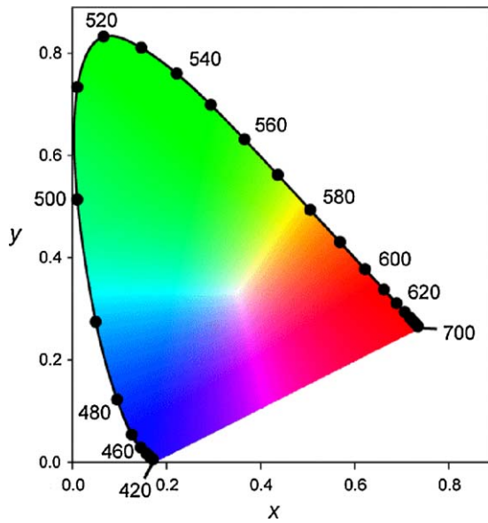
Figure 2 CIE 1931 (x, y) chromaticity diagram [10].
