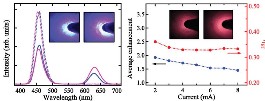
Figure 19 QD emission enhancement and energy-transfer efficiency of the hybrid color-conversion LED. (a) QW emission of the bare shallow-etched LED (dotted blue line) and the bare deep-etched LED (dotted pink line) at 3.8 and 7 mA, respectively. The solid blue line (solid pink line) represents the corresponding EL of the hybrid QD/shallow-etched LED (hybrid QD/deep-etched LED). Inset: left (right) panel shows emission of the hybrid shallow etched (deep-etched) LED for injection currents that produce the same QW emission intensity in the absence of QDs. (b) Red solid circles represent the effective nonradiative energy transfer efficiency versus the deep-etched LED injection current. Blue solid circles represent the enhancement of the QD emission. Inset: left (right) panel shows the emission of the QDs only in the hybrid shallow-etched (deep-etched) LED. Reprinted with permission from Reference [49]. Copyright 2010 WILEY-VCH Verlag GmbH & Co. KgaA, Weinham.
