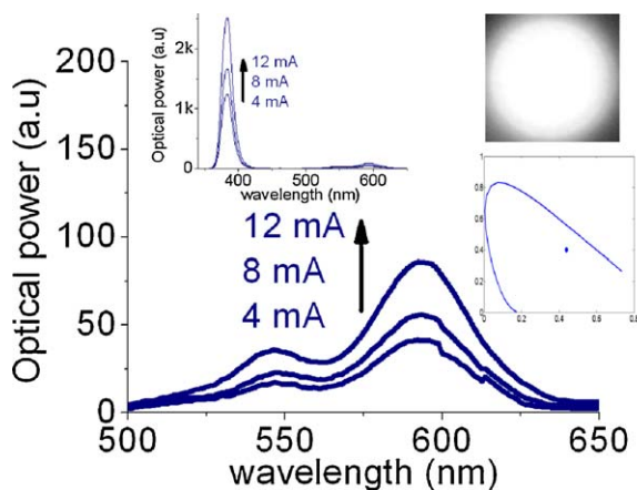
Figure 22 Luminescence spectra of mixed green and red-emitting CdSe/ZnS core/shell nanocrystals integrated on a near-UV InGaN/GaN LED. Insets show the evolution of the optical power with increasing current injection, a true color image of the hybrid LED, and its (x, y) tristimulus coordinates [52].
