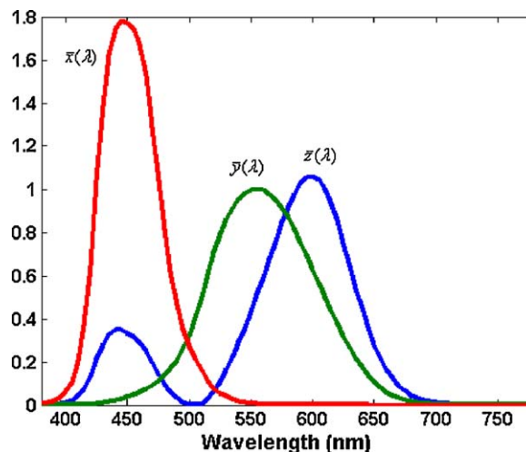
Figure 1 Spectral distribution of color matching functions [9].
