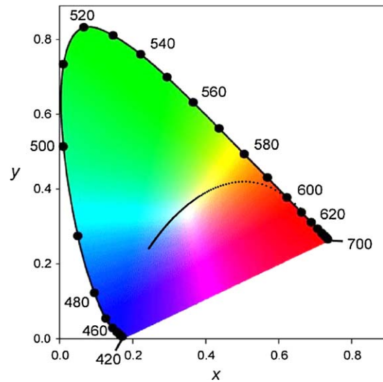
Figure 3 Planckian locus shown in the (x, y) chromaticity diagram [10].
