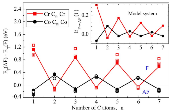
FIG. 1. (Color online) Energy difference of the AF and the F states in the \text{CrC}_n\text{Cr} and \text{CoC}_n\text{Co} atomic chains as a function of the number of C atoms. The ground state is AF for negative values of the energy difference. The solid, open, and crossed symbols represent the results of VASP, 16 SIESTA, 20 and GAUSSIAN03 21 calculations, respectively. The inset shows similar variations obtained in a model system.
