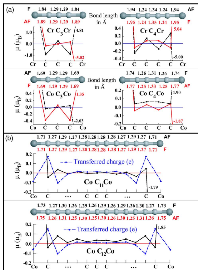
FIG. 2. (Color online) (a) Molecular structure and atomic magnetic moments in isolated \text{CrC}_n\text{Cr} and \text{CoC}_n\text{Co} chains for n=3 and 4 in their AF and F states. The values of the moments on the TM atoms are also denoted. (b) Same for longer chains. The charge transfer and induced atomic moments are plotted only in the ground states.
