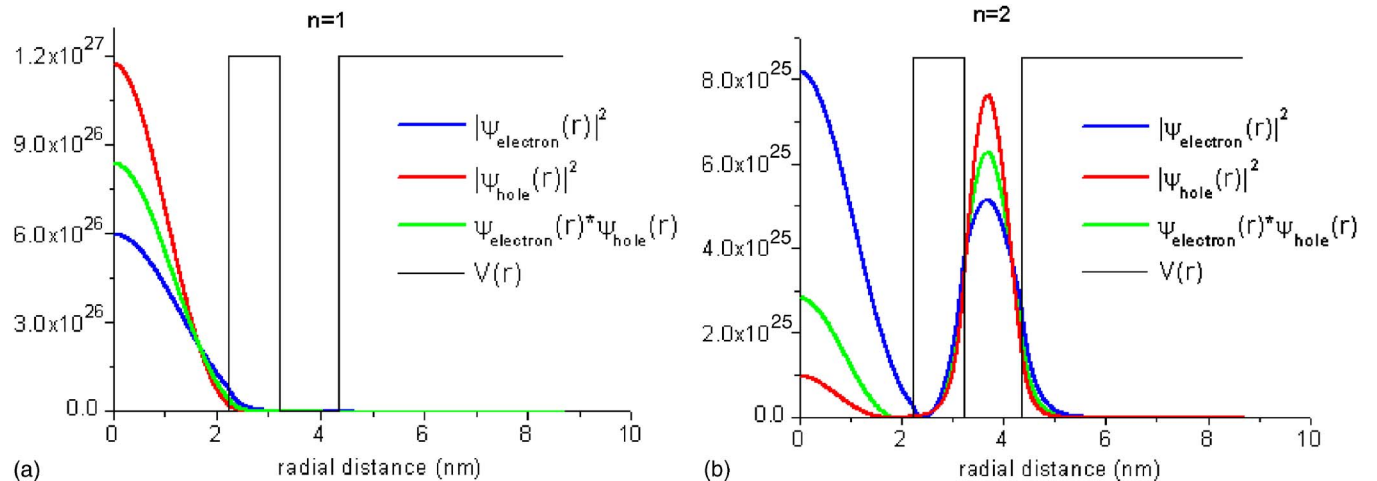
FIG. 2. (Color online) |\psi_{\text{electron}}(r)|^2 (in blue) and |\psi_{\text{hole}}(r)|^2 (in red) show the probability distribution of electron and holes in the (CdSe)ZnS/CdSe (core)/shell heteronanocrystals, respectively, while \psi_{\text{electron}}(r) * \psi_{\text{hole}}(r) (in green) indicates the relative spatial localization of excitons, with respect to the potential profile (in black): (a) for the ground states ( n=1 ) and (b) for the first excited states ( n=2 ).
