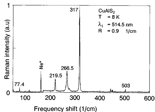
FIG. 4. The overall Raman spectrum of \text{CuAlS}_2 obtained at 8 K in the backscattering configuration from (112) plane for parallel polarization of the incident and scattered light. The excitation wavelength is 514.5 nm and spectral resolution 0.9 \text{cm}^{-1} . Notice again the large intensity of the \Gamma_1 phonon mode at 317 \text{cm}^{-1} .
