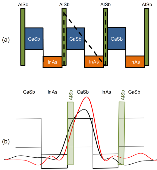
FIG. 1. (a) Conduction and valance band profiles for the proposed T2SL “N” structure. (b) Overlap integral with (red line) and without (black line) AlSb barrier under 0.001 meV bias. Negative bias is applied to the right side of the structure.
