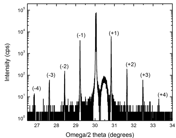
FIG. 2. High resolution x-ray diffraction curves of the superlattice along the 004 direction. Narrow FWHM of the peaks and highly ordered diffraction indicates uniform superlattice periods throughout the grown epilayer and excellent crystalline quality.
