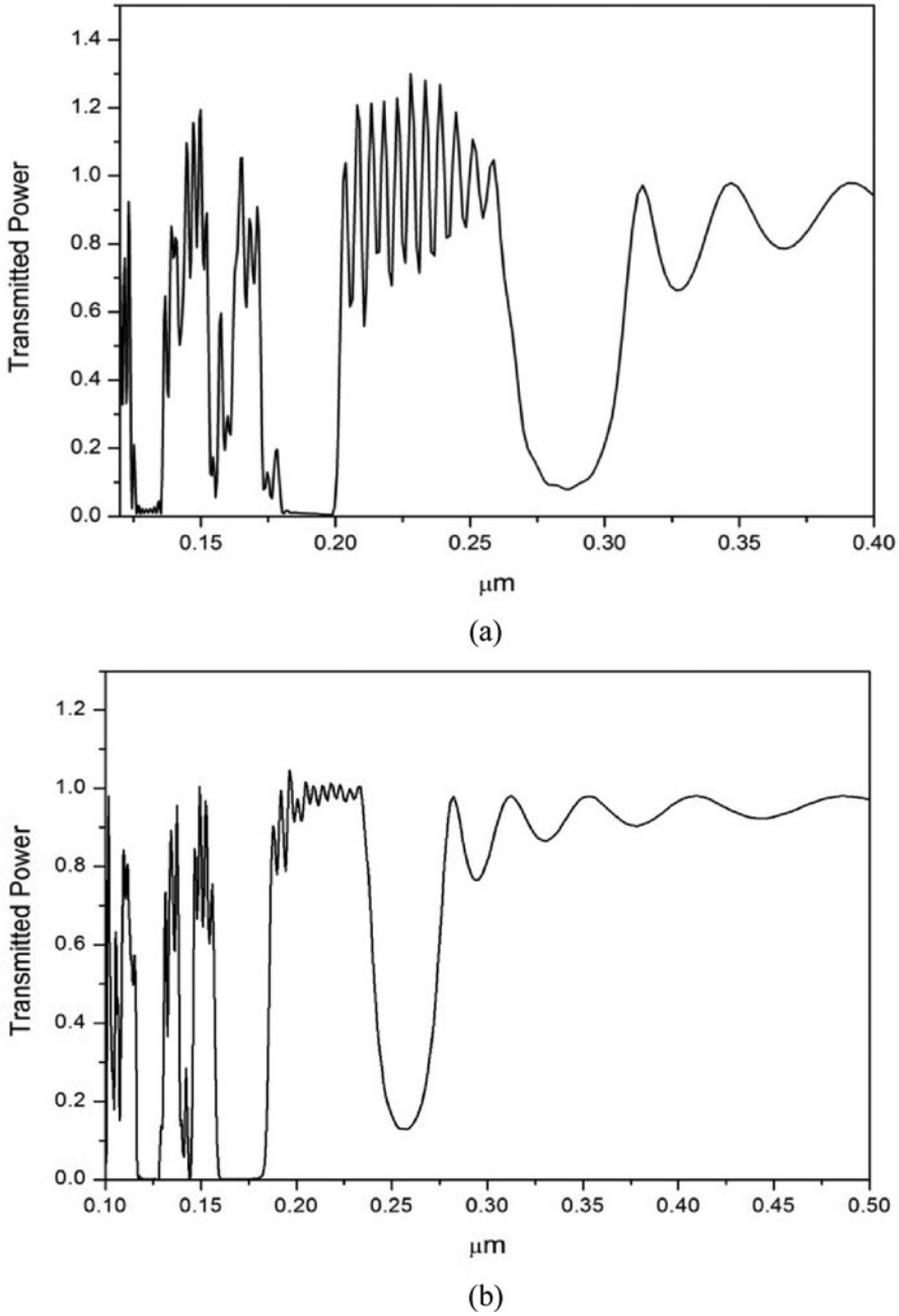
Figure 4. Transmitted power spectrum of LiNbO 3 PCLs on Al substrate: cylinders (a) and spheres (b).
