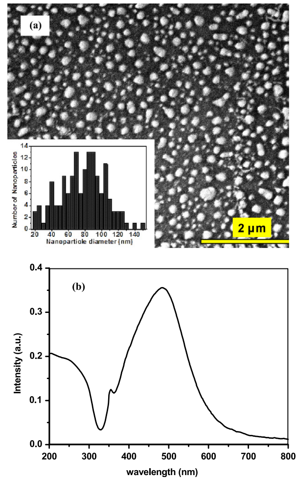
Figure 2. (a) SEM image, Ag islands on quartz glass, inset: size distribution of Ag islands. (b) UV–vis absorption spectrum of Ag islands on quartz.
