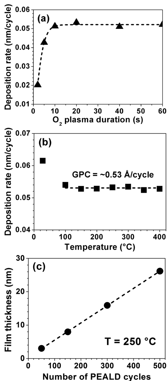
FIG. 1. Growth rate of Ga 2 O 3 thin films as a function of (a) O 2 plasma flow duration at 250 °C, and (b) deposition temperature. TMG dose and O 2 plasma flow rate were constant at 0.015 s and 25 sccm, respectively. (c) Ga 2 O 3 film thickness as a function of the number of PEALD cycles.
