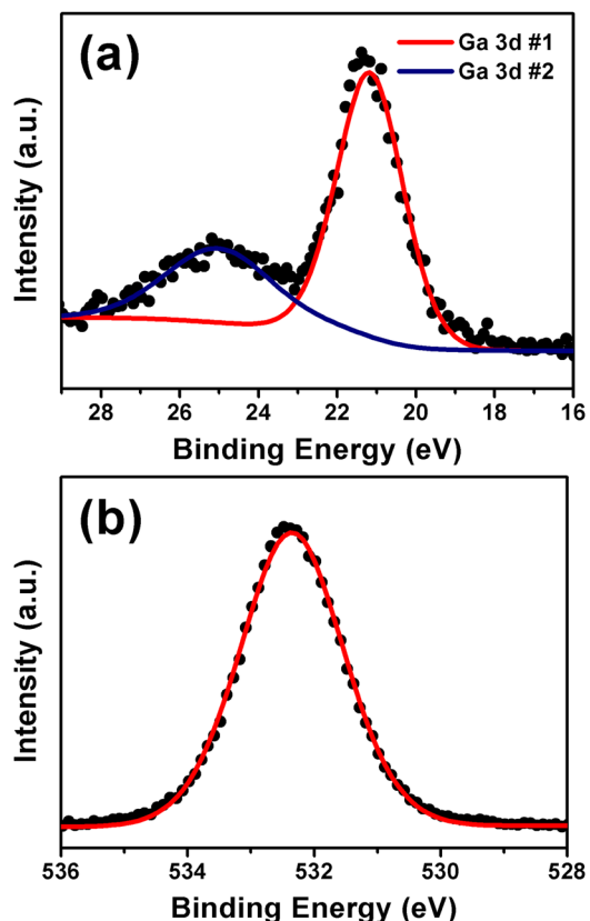
FIG. 2. (Color online) (a) Ga 3d and (b) O 1s high resolution XPS scans of \sim 26 \text{ nm} thick Ga 2 O 3 thin film deposited at 250 °C.
