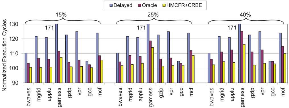
Fig. 12. Normalized execution cycles for various percentages of affected cache lines and TLB entries. The percentages of affected lines and entries vary from 15% to 25% to 40%.
