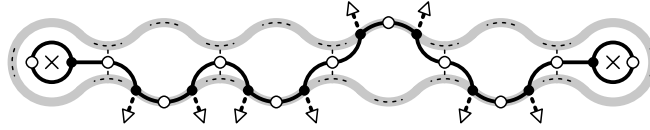
FIGURE 12. A junction of six M -cubics (*\uparrow\uparrow\downarrow\downarrow*)
