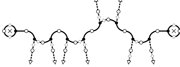
FIGURE 13. Necklace base points in the skeleton
