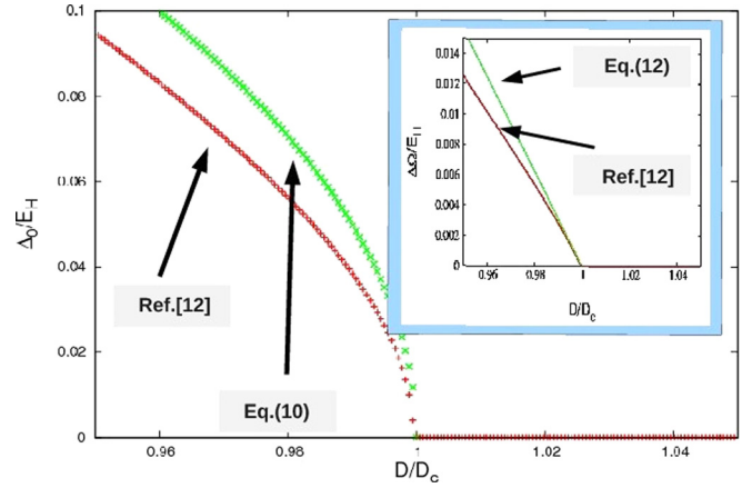
FIG. 1. Comparison of Ref. 12 with Eqs. (10) and (12) as D is varied near D_c . The main figure depicts \Delta_0/E_H and the inset is \Delta\Omega/E_H , where E_H = e^2/(4\pi\epsilon a_B) and a_B = \hbar^2 4\pi\epsilon/(e^2 m_x) . (The numerical solution includes the self energies as well as their realistically different masses.)
