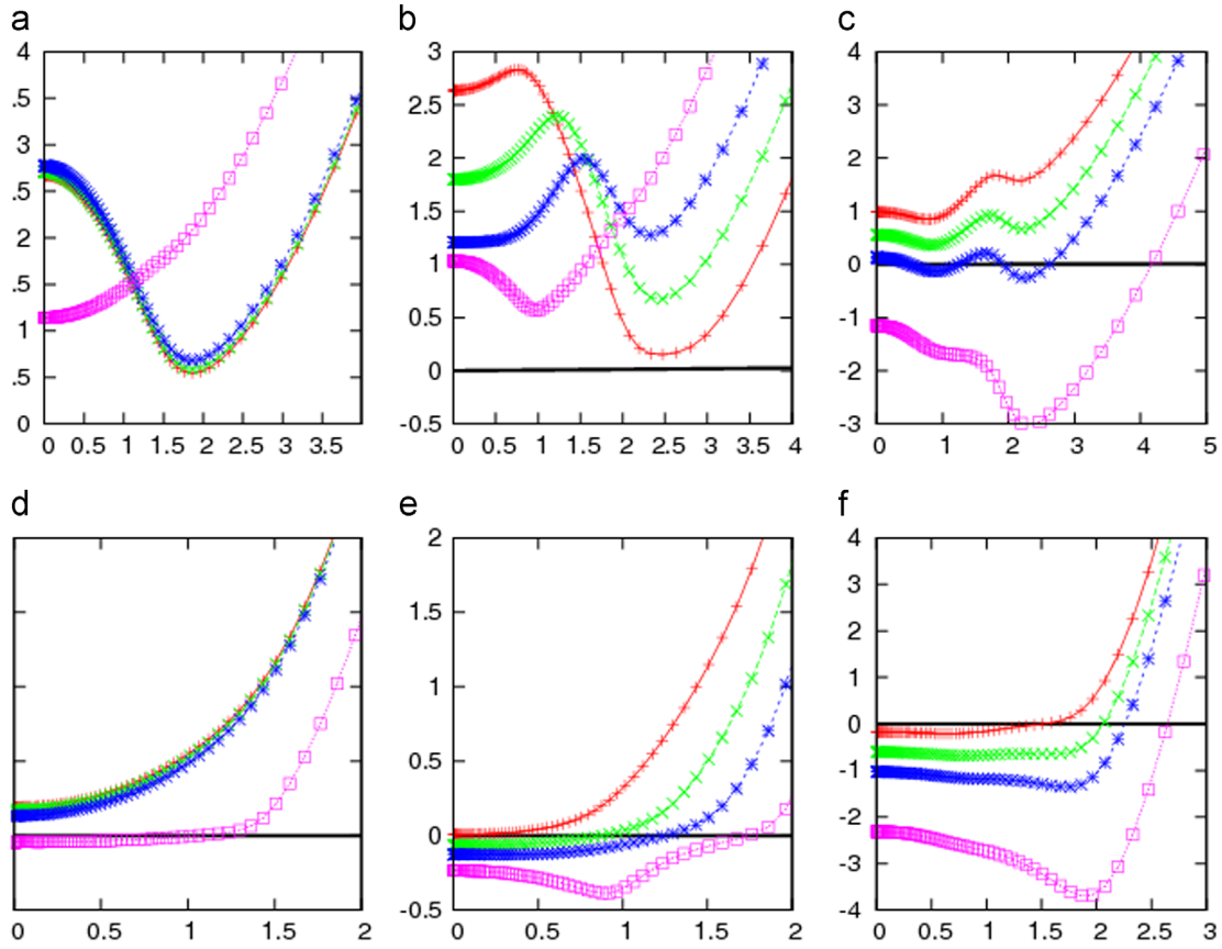
Fig. 2. The same as Fig. 1 for n_- \neq 0 . The upper and lower branches: (a) and (d) at B=0 , n_x a_B^2 = 0.55 and n_- = 0, 0.12, 0.36, 0.51 (from top to bottom at k=0 ); (b) and (e) at n_x = 1.5 and for n_- a_B^2 = 0, 0.36, 0.72, 1.44 at B=0 (from top to bottom at k=0 ); (c) and (f) at n_x a_B^2 = 1.5 and n_- = 1.1 for g^* B/B_0 = 0, 0.2, 0.4, 1.0 (from top to bottom at k=0 ).
