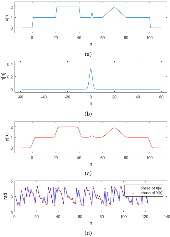
Fig. 1: (a) A 1-D signal x , (b) Gaussian filter h with \sigma = 1.2 , (c) filtered signal y = h * x and, (d) FT phase of x and y obtained using an FFT with size 128.
