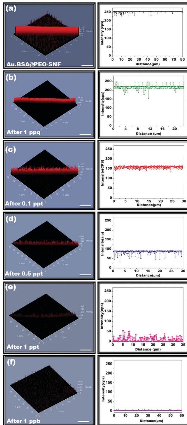
Fig. 3 CLSM images of Au.BSA@PEO-SNF upon exposure to different concentrations of TNT and their intensity profiles collected from the surface of the nanofiber (scale bar 10 \mu m).
