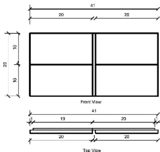
Fig. 4. Dimensions of the model.
