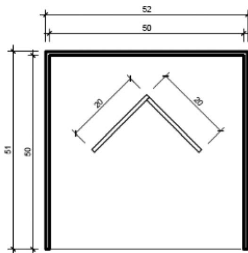
Fig. 5. Inside of the experiment box as a sectional top view.
