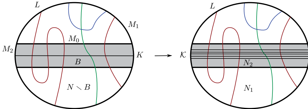
Fig. 3. This diagram represents the pairs (N, D \cup F) and (N, \mathcal{D} \cup F) . The gray band is the four ball N_2 = B = D \times B^2 .
