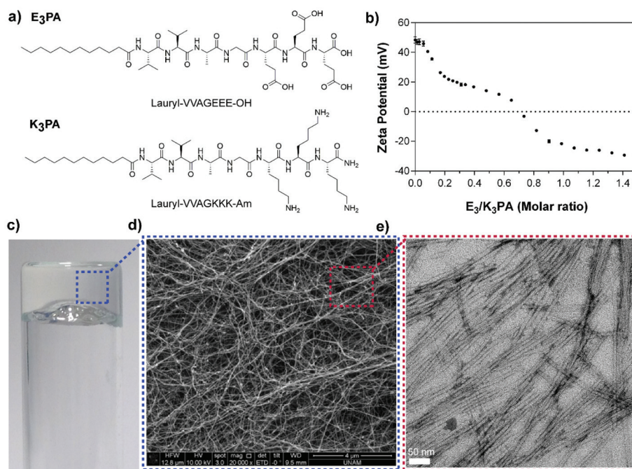
Fig. 1 (a) Chemical representations of E 3 PA and K 3 PA molecules, (b) the zeta potential change of the E 3 PA upon addition of K 3 PA at pH 7.4 in water, (c) the supramolecular PA network showing self-supporting gel properties, and (d) SEM and (e) TEM images of the coassembled PA nanonetwork and nanofibers, respectively.
