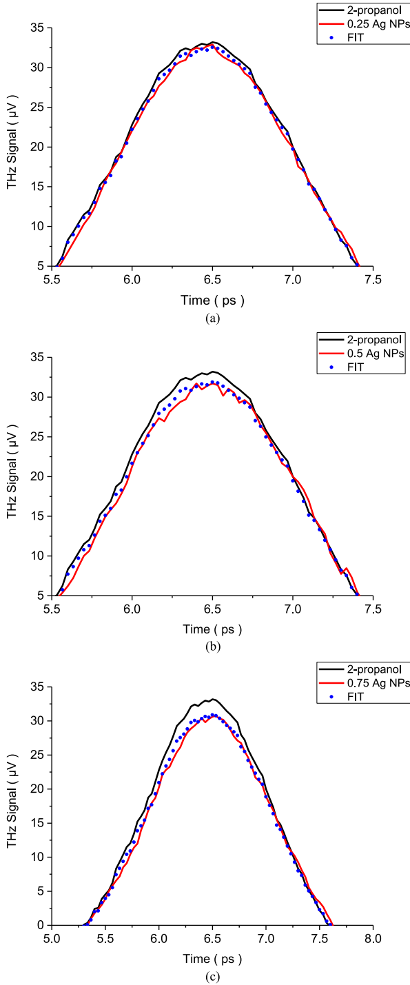
Fig. 4. THz time domain spectrum of Ag-NPs dispersions of Ag-NPs and 2-propanol reference waveform. The closed circles represent the matching fit respectively for NP volume ratio of (a) 0.25, (b) 0.5, and (c) 0.75.
