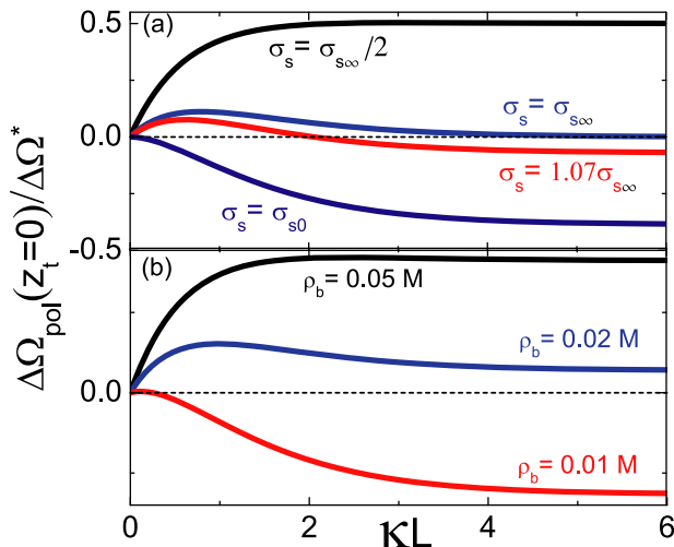
FIG. 8. The electrostatic grand potential of Eq. (35) on the membrane surface rescaled by the characteristic energy \Delta\Omega^* of Eq. (17) versus the adimensional polymer length \kappa L for various (a) surface charges and (b) salt densities at the permittivity \epsilon_m = 0 . In (a), the salt density is \rho_b = 0.01 \text{M} and in (b), the surface charge is \sigma_s = 0.1 \text{ e/nm}^2 .
