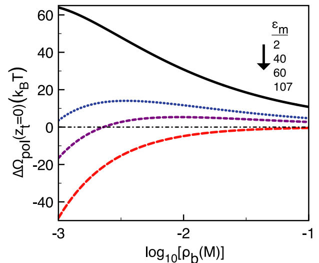
FIG. 9. The electrostatic grand potential at the membrane surface (Eq. (41)) versus the bulk electrolyte density \rho_b at the membrane charge \sigma_s = 0.01 \text{ e/nm}^2 for various membrane permittivities given in the legend. The remaining model parameters are the same as in Fig. 2.
