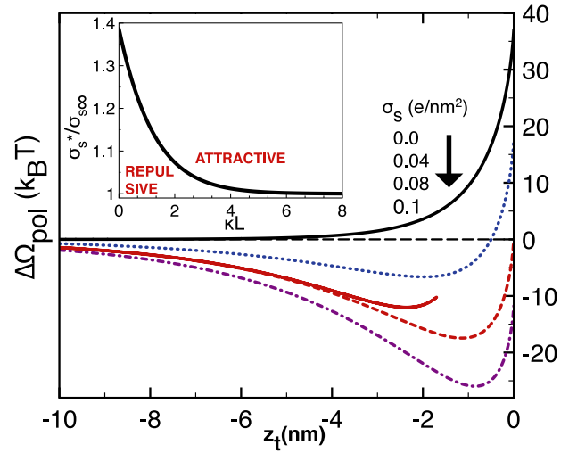
FIG. 7. Main plot: The electrostatic grand potential profile (Eq. (33)) at membrane permittivity \varepsilon_m = 0 , polymer length L = 1.0 \text{ }\mu\text{m} , salt density \rho_b = 10^{-2}\text{M} , and various surface charges as displayed in the legend. The solid red curve is from the asymptotic large distance law of Eq. (34). Inset: Characteristic surface charge (Eq. (36)) separating the attractive and repulsive membrane regimes rescaled by the long polymer limit of Eq. (38) against the adimensional polymer length \kappa L . The remaining model parameters are the same as in Fig. 2.
