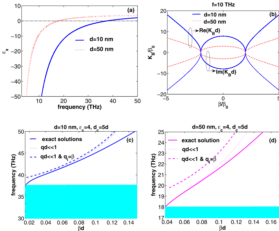
FIG. 3. Panel (a) shows dispersion of the “x” component of the effective permittivity of graphene metamaterial for d = 10 nm (solid curve) and d = 50 nm (dotted curve), where \epsilon_z = \epsilon = 4 . Panel (b) represents the hyperbolic dispersion of the GMMs at 10 THz. Dispersion of Tamm SPs of the GMM with d = 10 nm in the presence of a cap layer with \epsilon_c = 4 and d_c = 5d is represented in panel (c) with solid (exact answers), dotted (long-wavelength approximation), and dashed (long-wavelength approximation together with nonretarded one) curves. Panel (d) is similar to panel (c), but for d = 50 nm.
