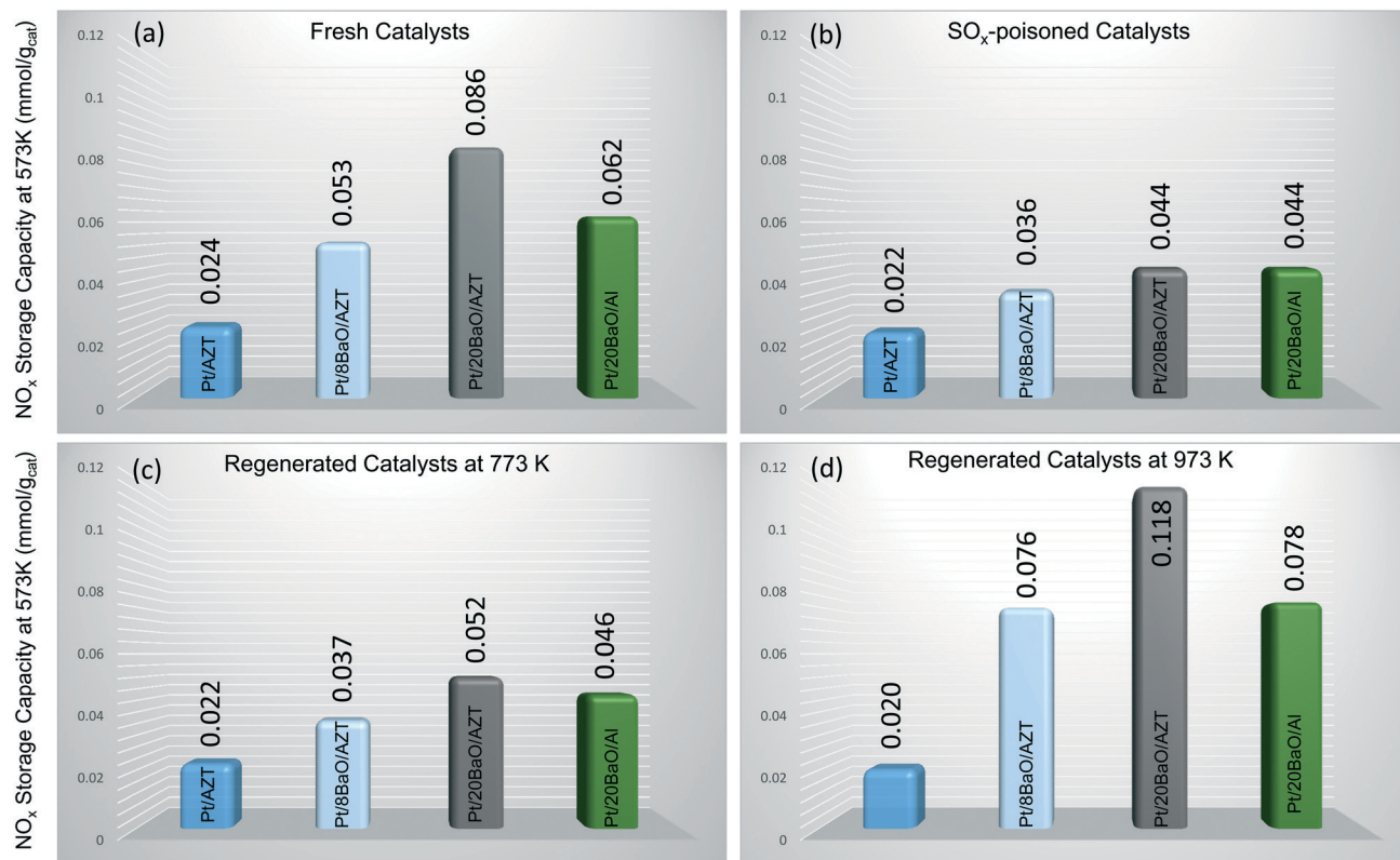
Fig. 7 NO x storage capacities (NSC) of Pt/20BaO/Al, Pt/8BaO/AZT, Pt/20BaO/AZT and Pt/AZT monolithic catalysts obtained via flow-reactor experiments at 573 K with an inlet gas feed of 500 ppm NO, 5% O 2 , 5% CO 2 , 5% H 2 O, balanced in Ar. NSC for (a) fresh catalysts, (b) after SO x poisoning, (c) after SO x poisoning and subsequent regeneration at 773 K, and (d) after SO x poisoning and subsequent regeneration at 973 K.
