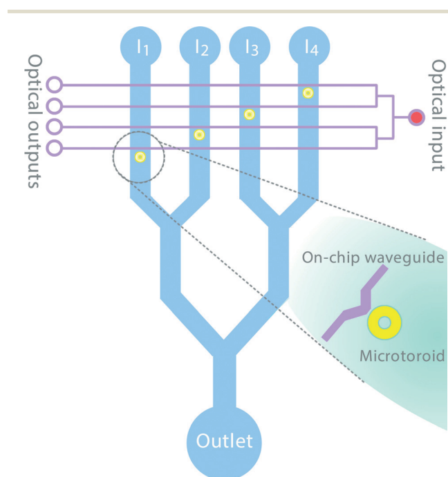
Fig. 3 Multiplexed oligonucleotide-based detection using microtoroids as optical resonators having high- Q factors. Illustration of a lab-on-a-chip biosensing system consisting of microfluidic channels each having one microtoroid (yellow circles), which can be used for multiplexed oligonucleotide-based detection. The proposed system has four inlets (from I_1 to I_4 ) and one outlet for controlled target flow in small volumes. Data are gathered separately from optical outputs, which are all branched from a common optical input (red lines). The inset shows an on-chip, curved waveguide and a microtoroid located at a critical distance as a schematic drawing regarding a previous work. 28
