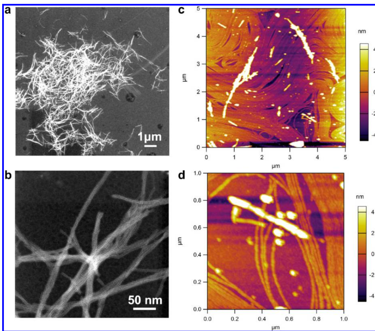
Figure 6. Imaging of n/p-coassembled CTC. STEM images (a and b) and AFM images (c and d) of n/p-coassembled supramolecular nanowires.
