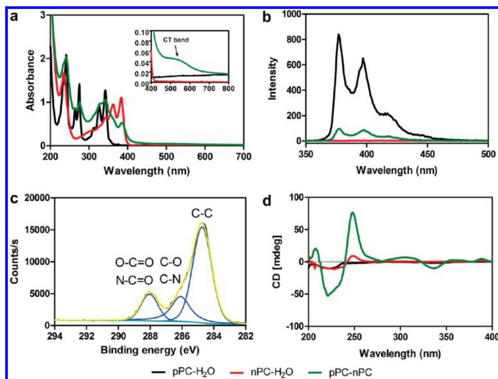
Figure 3. Spectroscopic characterization of pPC and nPC coassembly. (a) UV-vis absorption spectra and inset shows appearance of CT band. (b) Fluorescence emission spectra (excitation wavelength = 340 nm) of pPC-nPC CT complex. (c) XPS analysis (Gaussian deconvolution of the C 1s signal) of pPC-nPC powder and (d) CD spectra of pPC and nPC coassembly in aqueous media.
