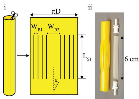
C) Illustration of the SLiT design parameters
