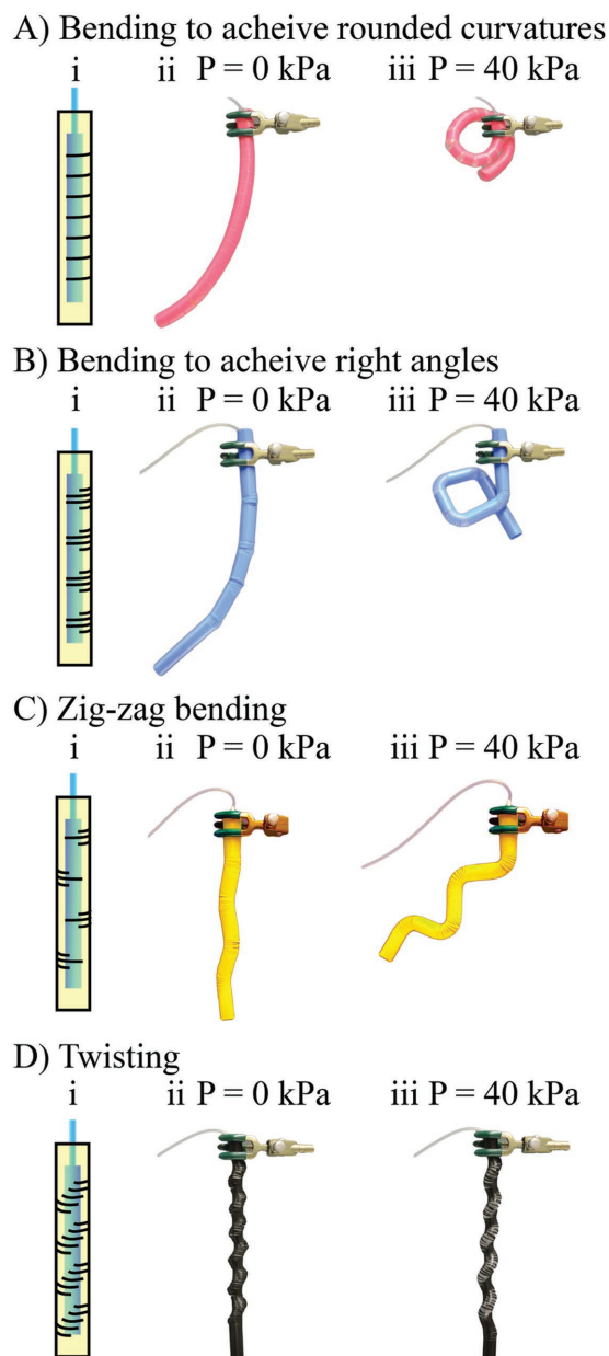
Figure 3. Actuators with horizontal slits that produce different types of motions, where i) is the schematic illustration of the actuator and slits, ii) is the photograph of unactuated system and iii) is the photograph of the actuated system pressurized to 40 kPa. Parts (A) and (B) show actuators that can curl with different curvatures. Part (C) shows an actuator that bends in a zig-zag manner. Part (D) shows an actuator that can twist and extend simultaneously.
