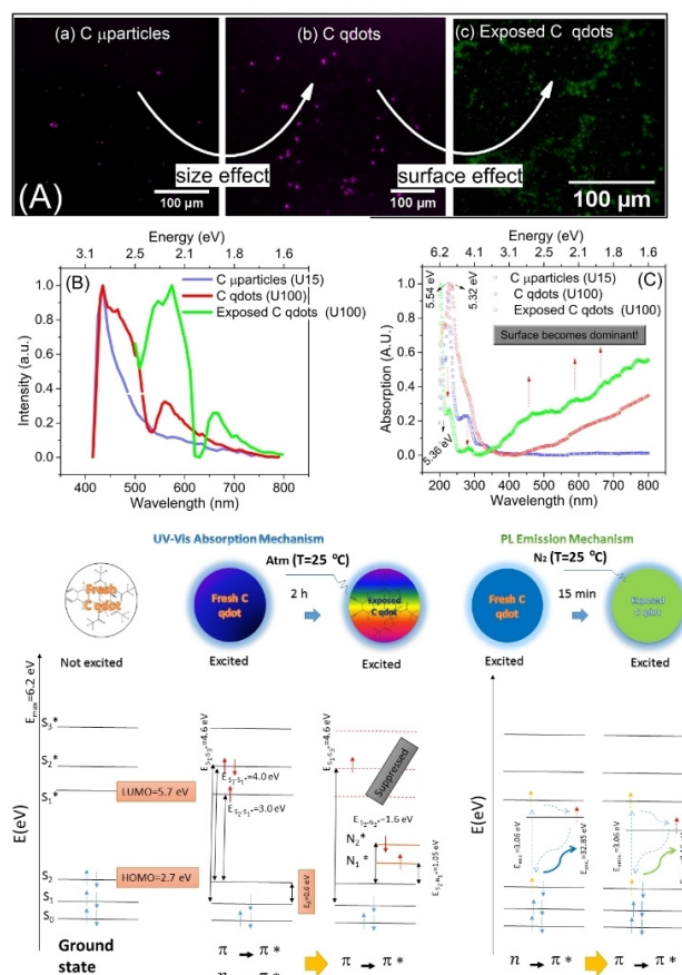
Figure 7. Size and surface effects on the light emission properties of C qdots. (A) LSCM images of (a) U15, (b) as-prepared U100 sample and (c) the N 2 exposed U100 sample, (B) corresponding photoluminescence results at the excitation wavelength of 405 nm and (C) the UV-Vis absorption spectroscopy data are shown. The possible mechanisms are schematically demonstrated. The size effect shows an intensification in the PL emission due to increase in the number of n \rightarrow \pi^* transitions. The surface states were formed due to N atoms caught by C molecules in the C qdot surface which in return would result in the red shift in the PL emission attributed to the transformation from n \rightarrow \pi^* transition to \pi \rightarrow \pi^* transition.
