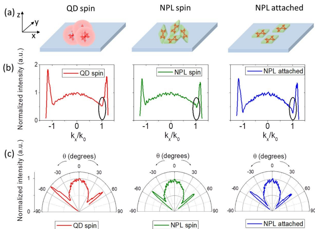
Figure 5. Angle and k -space dependent p-polarized emission characteristics of spin-coated spherical QDs, spin-coated NPLs, and attached NPLs. (a) A schematic representation of film of spin-coated QDs, spin-coated NPLs and NPLs via linker-based attachment on glass substrates. (b) k -dependent and (c) \theta -dependent intensity profile of p-polarized spectra of all samples. k_0 is the wavevector in air. Angle-dependent polar plots were obtained by performing Jacobian conversion on the k -space spectra. The substrate is on the x - y plane. The plane of incidence for the emitted light is on the x - z plane. The collected radiation emitted in the x - z plane (defined as p-polarized) emanates from a distribution of emitter dipoles oriented in-plane ( p_x ) and out-of-plane ( p_z ) of the substrate.
