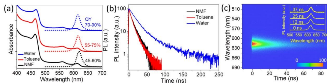
Figure 3. Steady-state and time-resolved PL measurements of the NPLs in different solvents.
