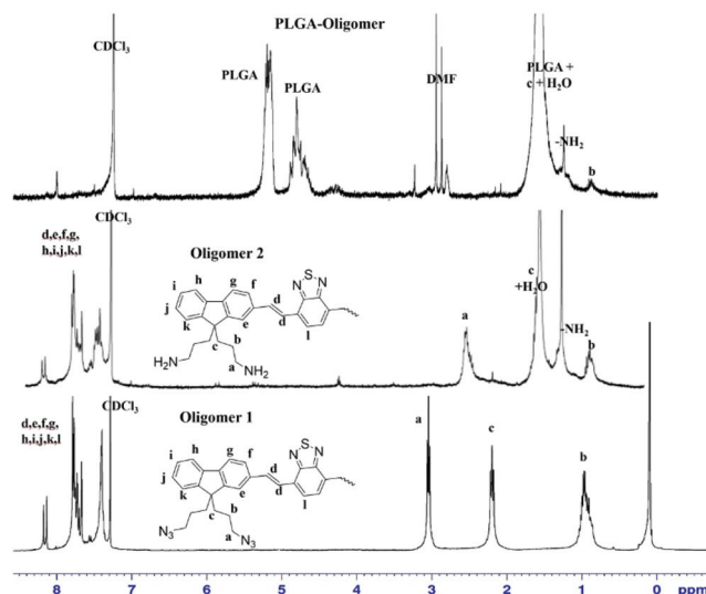
Fig. 1 1 H-NMR (400 MHz, CDCl 3 , 25 °C) spectra of Oligomers 1, 2 and PLGA-Oligomer.
