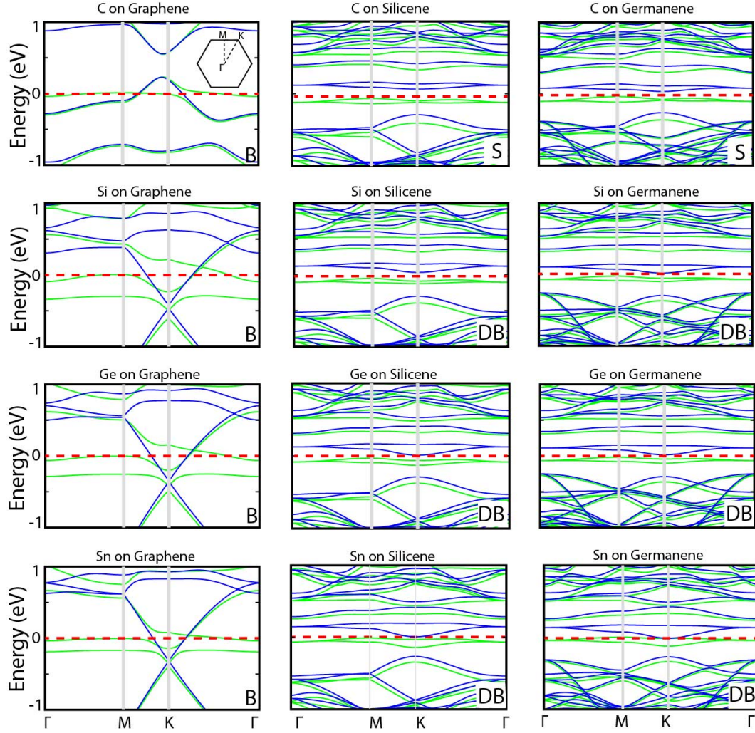
Figure 4: Electronic band structures of monolayer graphene, germanene, and silicene with adatoms C, Si, Ge and Sn, which form a 5 \times 5 supercell or pattern. In the spin polarized systems, spin up and spin down bands are shown with green and blue lines. The zero of energy shown by red dashed line is set to the energy of highest occupied state. Binding structures (as B, S, DB) are indicated in each panel. Brillouin zone and symmetry directions are shown by inset.
