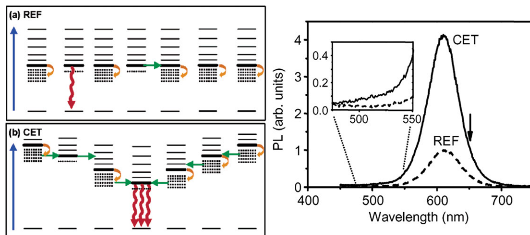
Figure 2 Two different QD structures are described: (a) Nonscattered reference (REF) structure and (b) cascaded energy transfer (CET) structure. (b) The CET structure consists of graded layer-by-layer assembled green/yellow/orange/red/orange/yellow/green QDs. (a) The REF structure consists of layered red QDs. On the left, electronic energy levels of the graded QD-employing CET structure and the only red-emitting QD-employing REF structure are shown. On the right, steady-state PL emission is depicted for the both structures. The CET structure exhibits substantial enhancement in the PL emission as compared with the REF structure due to the trapped exciton recycling effect. [Reprinted (adapted) with permission from ref. [69] (Copyright 2004 American Chemical Society).]
