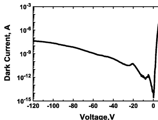
FIG. 1. Current voltage measurements of a photodetector with a 200 \mu\text{m} diameter.
