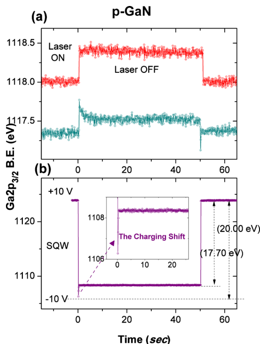
FIG. 4. (Color online) (a) The same data as presented in Fig. 2(a) for the p-GaN. (b) The Ga 2p_{3/2} B.E. changes recorded in the transient mode with 0.1 s intervals, as the sample is subjected to SQW electrical pulses with 10 V amplitude and 0.01 Hz frequency and with the flood-gun turned-on. The inset shows the expanded version of the data.
