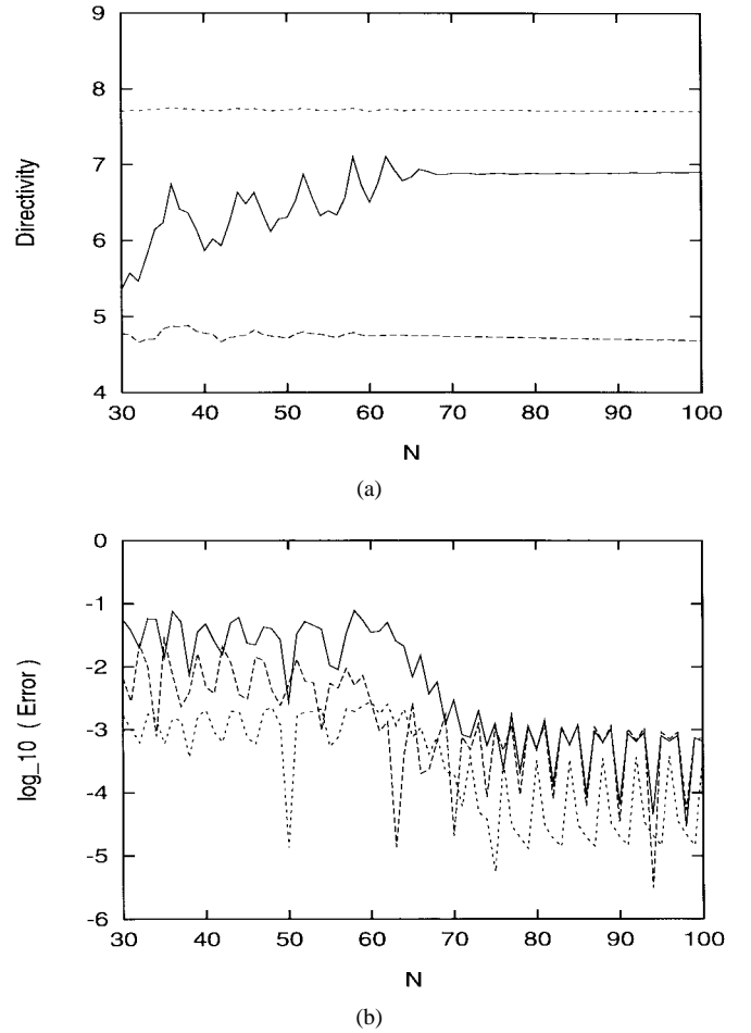
Fig. 2. (a) Directivity D_\beta and (b) its computational error \Delta D_\beta = \log_{10}(|D_\beta^N - D_\beta^{N+1}|/D_\beta^N) as functions of the truncation number N for a circular grating of M = 4 impenetrable metal strips with air slots (solid curves) and with dielectric shells characterized by \epsilon_r = 16 , h = 0.4\lambda_e (dashed curves), and by \epsilon_r = 16 + 0.5i , h = 0.5\lambda/\text{Re}(\sqrt{\epsilon_r}) (dotted curves). Other relevant parameters are Z/Z_0 = 0.1(1 - i) , \varphi_{ap} = 0.5^\circ , ka = 62.8 , r_0 = 0 , \beta = 0^\circ , and kb = 5 that corresponds to the beam halfwidth at half power \varphi_b = 21.4^\circ and to the source directivity in free space D_\beta = 7.82 .
