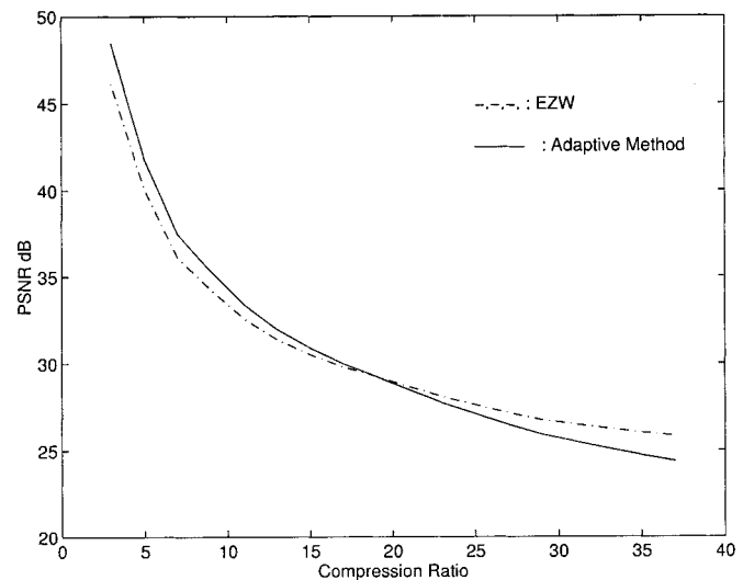
Fig. 14. EZW versus adaptive method at different CRs.
