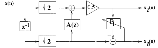
Fig. 8. Adaptive filter bank structure with an antialiasing filter.
