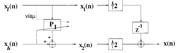
Fig. 3. Synthesis stage of the adaptive filter bank structure.
