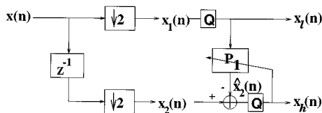
Fig. 16. Analysis stage of the adaptive filter bank structure with quantization.
