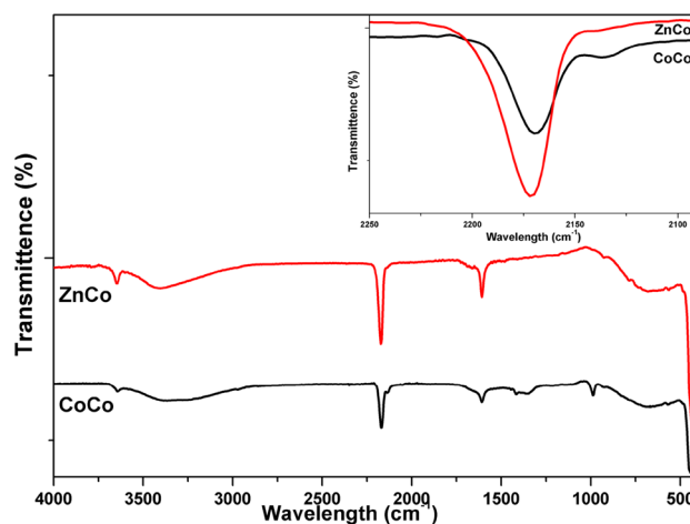
Fig. 1 FTIR spectra of bulk Co–Co (black) and Zn–Co (red) PBA. Inset: \nu(\text{CN}) stretches of Co–Co and Zn–Co PBA
