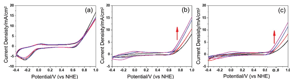
Figure 6. CVs of \text{m-LiMn}_{1.6}\text{Co}_{0.4}\text{O}_4 -# (# is 0, 1, 3, and 5) a) 1st set before CP, b) after 12 h CP at 1 \text{ mA cm}^{-2} , and c) after 12 h at 1 \text{ mA cm}^{-2} and 6 h CP at 10 \text{ mA cm}^{-2} .
