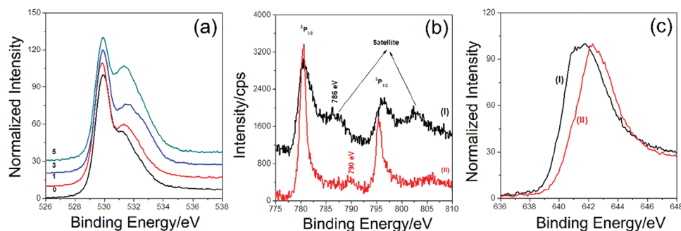
Figure 8. XPS spectra of electrode surface: a) O 1s region of \text{m-LiMn}_2\text{O}_4 -# (# is 0, 1, 3, and 5 as marked on the spectra) after 12 h CP experiment at 1 \text{ mA cm}^{-2} , b) Co 2p and c) Mn 2p ( 2\text{P}_{3/2} ) regions of \text{m-LiMn}_2\text{O}_4 -5 before (I) and after (II) CP experiment.
