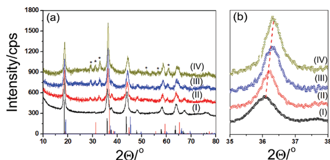
Figure 2. PXRD patterns of m-LiMn 2 O 4 -# a,b), where # is (I) 0, (II) 1, (III) 3, and (IV) 5 (the reference data in panel a): black lines-LiMn 2 O 4 , blue lines-LiCoO 2 , red lines-Co 3 O 4 , and *-Mn 3 O 4 .
