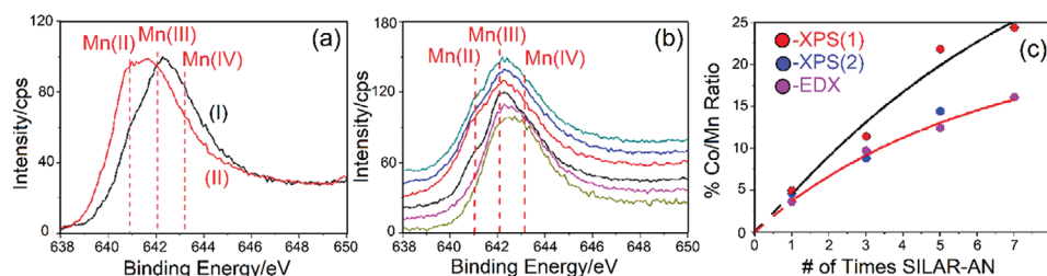
Figure 3. Mn 2p XPS spectra of: a) grind sample of m\text{-LiMn}_2\text{O}_4 (I) and the electrode top surface (II), b) bottom to top: m\text{-LiMnCoO}_4 (olive), m\text{-LiMn}_{1.5}\text{Co}_{0.4}\text{O}_4 (pink), and m\text{-LiMn}_2\text{O}_4 -# (# is 0 (black), 1 (red), 3 (blue), and 5 (green)), and c) percent Co/Mn from XPS (electrode surface, XPS(1) and grind sample XPS(2), and EDX data).
