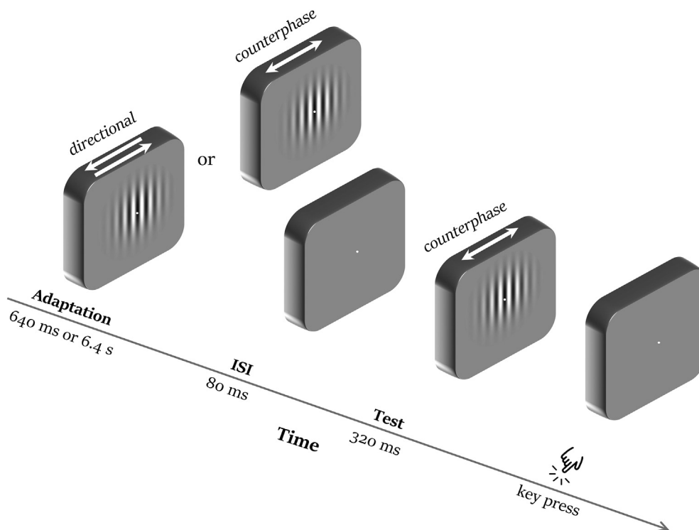
Fig. 1 – Schematic representation of the stimuli and timeline. In each trial, the adapting stimulus was shown first. The adapting pattern was either counterphase flickering or directional (leftward or rightward) and its duration (short: 640 msec or long: 6.4 sec) was varied across trials. After an 80 msec adapting-test blank interval, the counterphase flickering test pattern was displayed for 320 msec.
