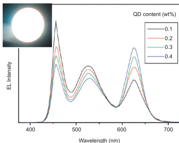
Figure 19 Spectra of a QD-WLED, which is designed using \text{Sr}_2\text{SiO}_4:\text{Eu} green phosphor and red QDs of \text{CdSe/CdS/CdZnS/ZnS} , at 30 mA with varying QD concentrations [73]. The inset shows a photograph of the device. Reprinted with permission from Ref. [73]. Copyright 2011 American Chemical Society.
