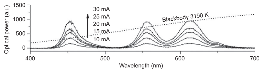
Figure 14 Measured spectra of the white LED fabricated by hybridizing CdSe/ZnS QDs on blue InGaN/GaN LED. This QD-WLED exhibits the following performance: CRI=81, LER=323 lm/W opt , and CCT=3190 K [64]. Reprinted with permission from Ref. [64]. Copyright 2008 American Institute of Physics.
