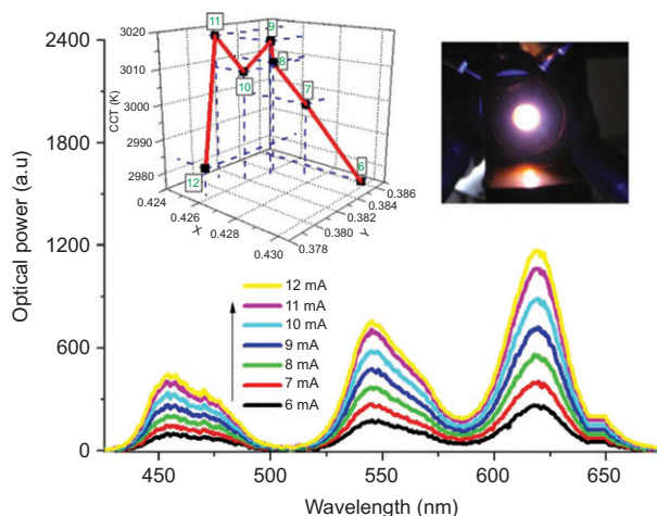
Figure 15 Measured spectra, chromaticity coordinates, and photograph of the CdSe/ZnS QD-integrated white LED exhibiting figure-of-merits of CRI=89.2, LER=357 lm/W opt , and CCT=2982 K [65].
