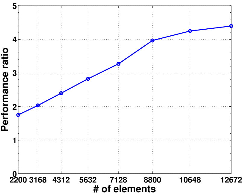
Figure 8: Performance ratio depending on the number of elements on channel.
