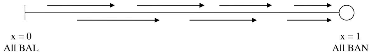
Figure 1 Homogeneous Population Monomorphic Equilibrium
