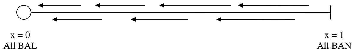
Figure 2 Homogeneous Population Monomorphic Equilibrium
