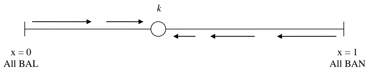
Figure 3 Homogeneous Population Polymorphic Equilibrium
