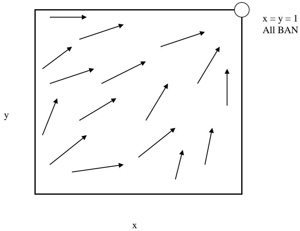
Figure 4 Non-homogeneous Population, Monomorphic Equilibrium
