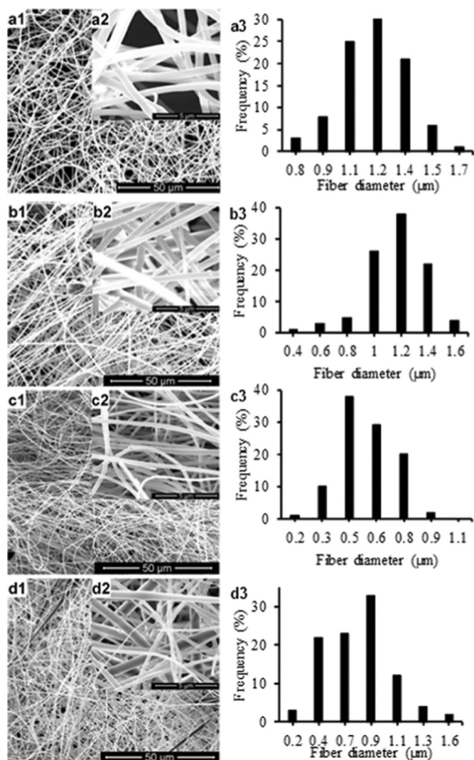
Fig. 6. SEM images of (a1) HP1(65% hydrolyzed), (b1) HP2 (86% hydrolyzed), (c1) HP3 (94% hydrolyzed) and (d1) HP4 (99% hydrolyzed). (a2–d2) higher magnifications (5 μm) and (a3–d3) fiber diameter distributions of corresponding samples.
