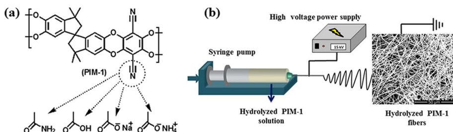
Fig. 1. a) Chemical structure of PIM-1 and possible hydrolysis products, b) illustration of the electrospinning process of hydrolyzed PIM-1 fibers.
