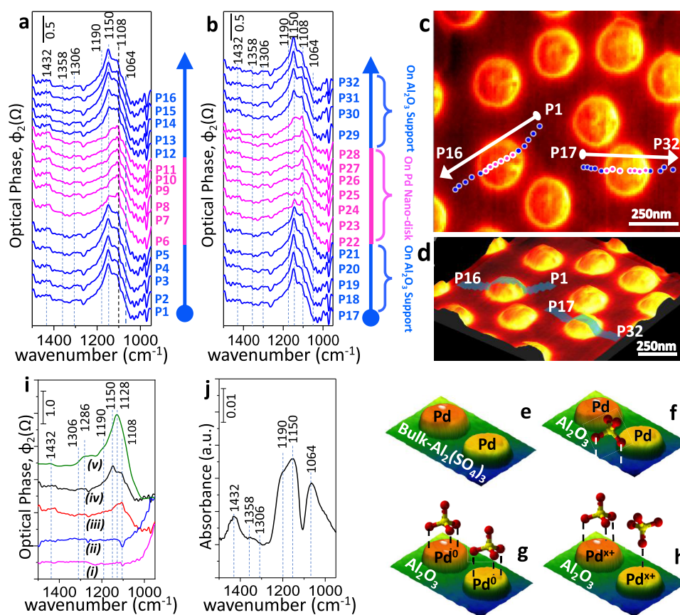
Figure 3. (a, b) Nano-FTIR spectra collected from the line scans across two independent mildly sulfur-poisoned single Pd nanodisks on Al 2 O 3 . Nano-FTIR spectra labeled with blue color were acquired directly from the Al 2 O 3 support sites (corresponding to points P1–P5, P12–P16, P17–P21, and P29–P32 in panel (c)), while the purple spectra were acquired directly from the Pd nanodisks (corresponding to points P6–P11 and P22–P28 in panel (d)). (c) 2D and (d) 3D representations of total IR-reflection s-SNOM images of the mildly sulfur-poisoned Pd(nanodisk)/Al 2 O 3 (thin-film) planar model catalyst surface showing the locations of the points where the nano-FTIR line scan spectra were acquired. (e–h) Schematic (not drawn to scale) illustration of the prominent sulfate species detected in the nano-FTIR spectra given in panels (a, b). (i) Nano-FTIR spectra obtained from: pristine Pd nanodisk (i) and pristine Al 2 O 3 (ii) domains of the clean Pd nanodisk/Al 2 O 3 (thin-film)/Si(100) surface, mildly sulfur-poisoned Pd nanodisk (iii), and mildly sulfur-poisoned Al 2 O 3 domains (iv) of Pd nanodisk/Al 2 O 3 (thin-film)/Si(100) surface, as well as the mildly sulfur-poisoned Al 2 O 3 (thin-film)/Si(100) surface that does not have any Pd disks (v). For spectra i, ii, and v, the nano-FTIR spectrum of the Si wafer was used as the background. Spectra i and ii were used as the background for spectra iii and iv, respectively. (j) Far-field ATR-IR spectrum of the identical mildly sulfur-poisoned Pd(nanodisk)/Al 2 O 3 model catalyst given in panels (a–i).
